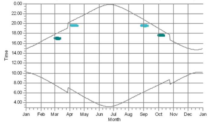
10: Shadow Receptor: 1.0 ä¼» 1.0 Azimuth: 0.0j° Slope: 90.0Ê½ (12)
